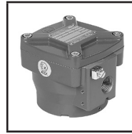
TYPE 08: NF / WSNF Aluminium; epoxy coated / AISI 316L SS EN/IEC 60079-1 and EN/IEC 60079-31
